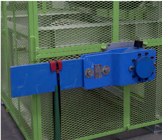
Low Speed Backstop FRHD 800 in Incline Conveyor
