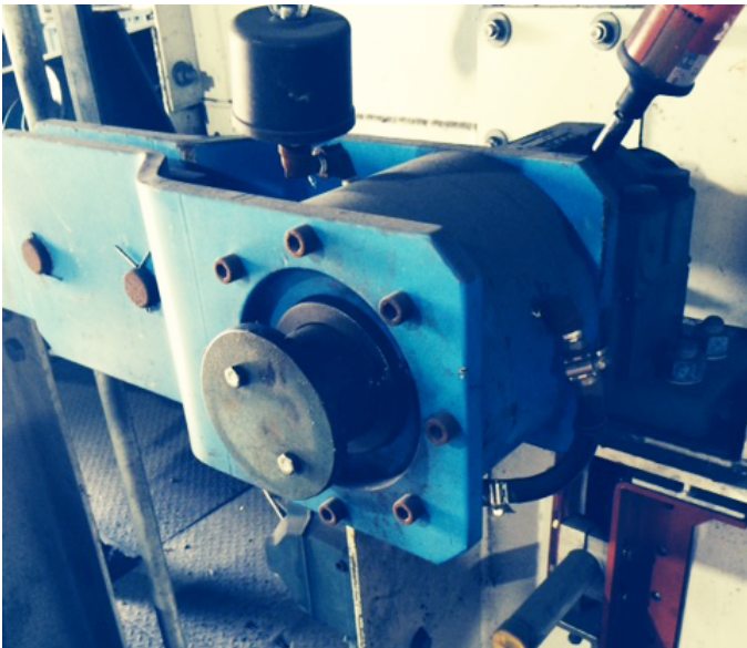
Low Speed Backstop FRHD 700 in Incline Conveyor
