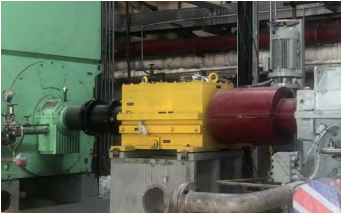
Housing Freewheel FHHS 18000 in water pump
